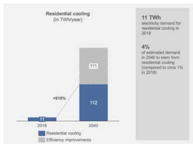
Figure 24 – Electricity demand from residential cooling in 2018 and 2040
